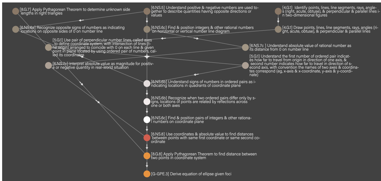
Figure 4: Visualization of one of the longest paths of the network: the entire prerequisite chain of G-GPE.3 Derive equation of ellipse given foci .
